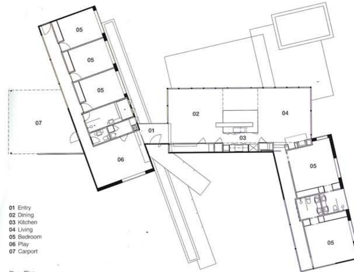
Floor Plan
